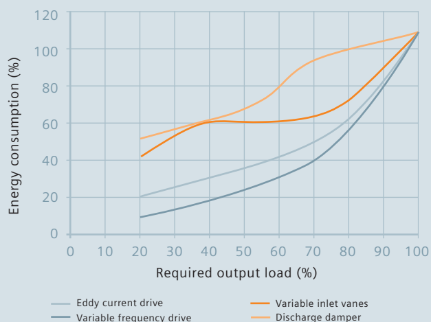
Electric drives market in HVAC industry: Energy consumption versus required output load (Europe), 2010
